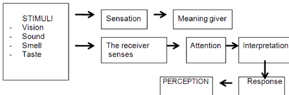
Figure 1. Perceptual process
