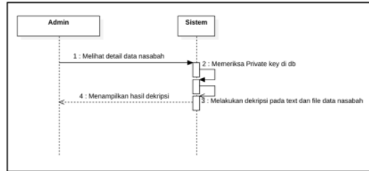
Gambar 3. Sequence Diagram Detail Data Nasabah.
