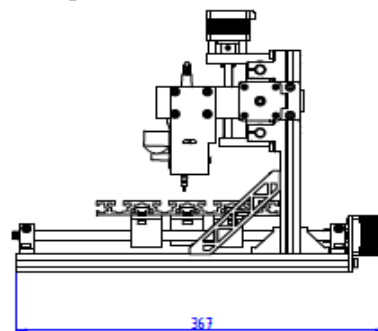
TAMPAK SAMPING
