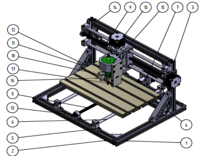
TAMPAK ISOMETRIK
