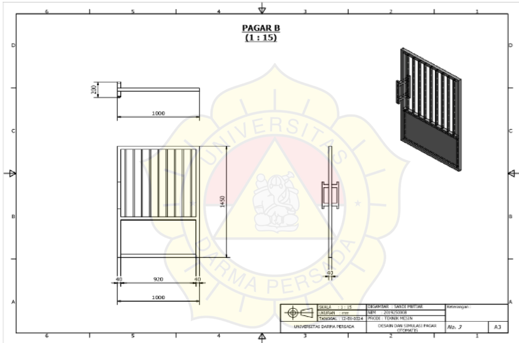
Gambar. Desain 2D Autodesk Inventor Professional
