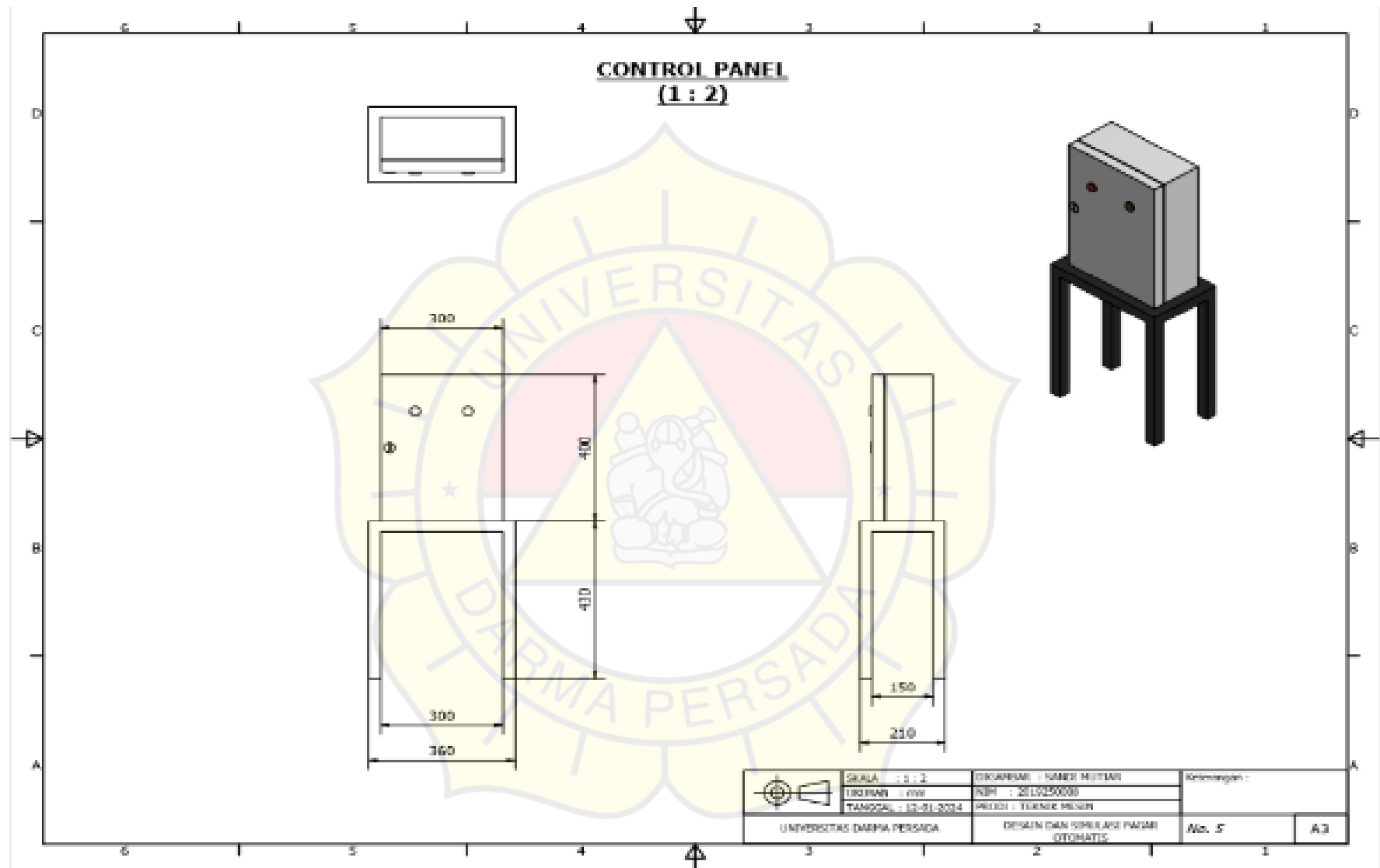
Gambar. Desain 2D Autodesk Inventor Professional
