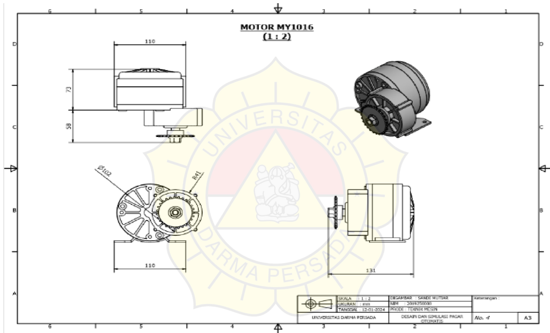
Gambar. Desain 2D Autodesk Inventor Professional
