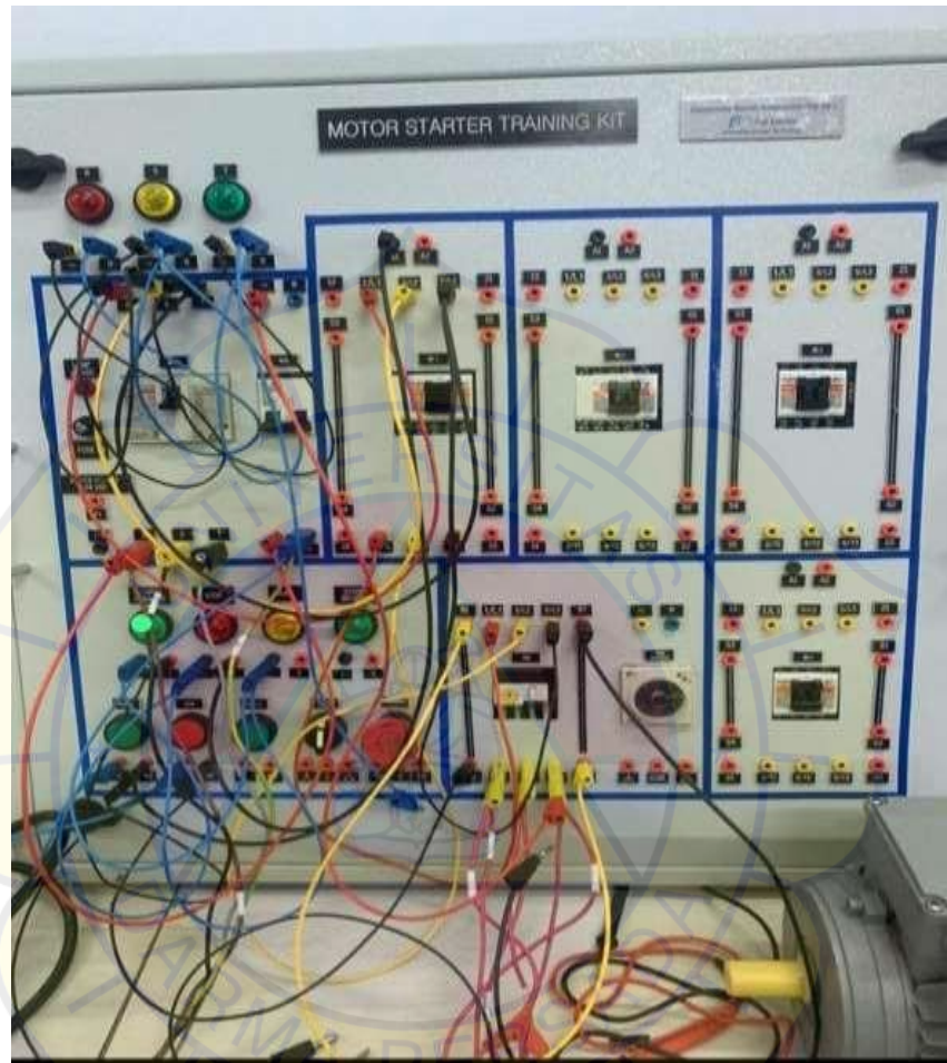
Lampiran 1 Gambar starter kit rangkaian direct on line
